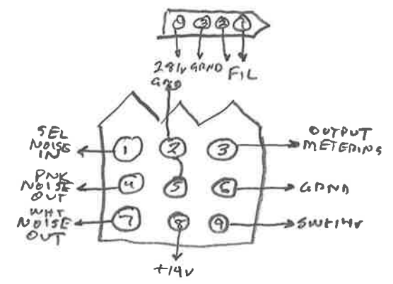
OUTSIDE CHASSIS VIEW
