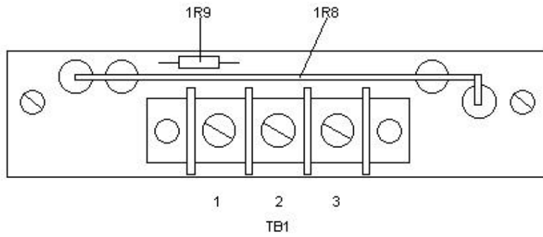
Charge Current Meter Shunt Assy
