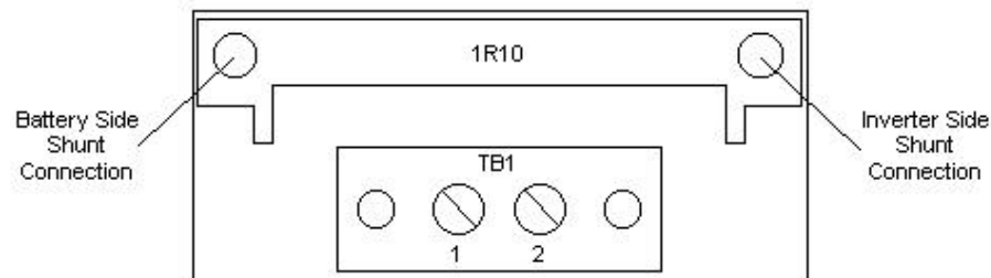
Inverter Current Meter Shunt Assy
